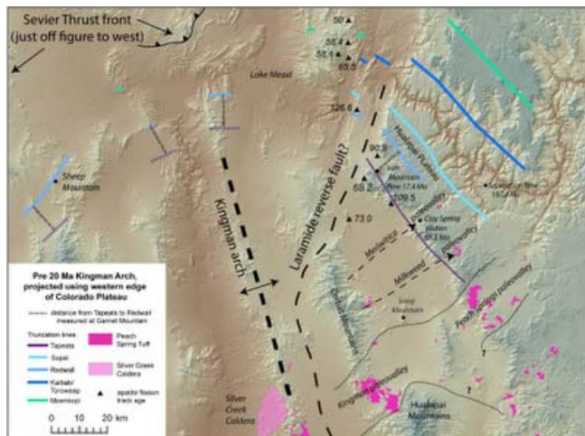
Image from Sue Beard and Jim Faulds workshop abstract showing the area of the Kingman Arch (heavy dashed line, left); three paleovalleys with their names trending onto the Colorado Plateau (small dashed lines); outcrops of the 18.5 Ma Peach Springs Tuff (dark pink) and its suspected source caldera (light pink); and the western end of the Grand Canyon (upper right). The parallel colored lines are the southwestern limit of various Grand Canyon strata.
