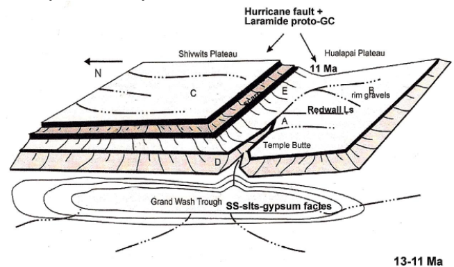
Figure 2: Young’s (2008) schematic of initial canyon incision at base of retreating Shivwits scarp; water drains to Grand Wash Trough. Tributary drainage on the Hualapai Plateau was parallel to regional dip and provided runoff for headward incision eastward. Rocks from Temple Butte to Redwall age were beveled across the northeast dipping structural slope on the Hualapai Plateau. The 13-11 Ma sandstone-siltstone-gypsum facies was supplied by Supai, Coconino, and Toroweap clastics
