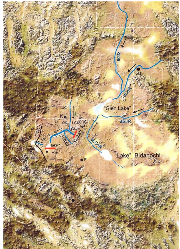
Figure 1: Proposed drainage on the Colorado Plateau with respect to the Grand Canyon area in the time frame of 17-11 Ma. F=Flagstaff, PS=Peach Springs, LV= Las Vegas, K=Kanab, GJ=Grand Junction, GWC=Grand Wash Cliffs, aGR=ancestral Green River, aCoR=ancestral Colorado River, aSJR=ancestral San Juan River, aLCoR=ancestral Little Colorado River, JC=Johnson Creek, C=Cedar Knoll, LCK=Little Cedar Knoll, GN=Goosenecks, RL halite=Red Lake halite, SS=Shivwits scarp. Between the red lines mark the route that the Colorado River still takes today. Base map from Blakey and Ranney (2008).
